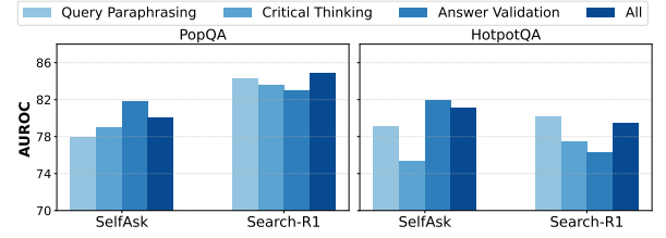
Figure 6: Performance of R^2C with different action sets.
